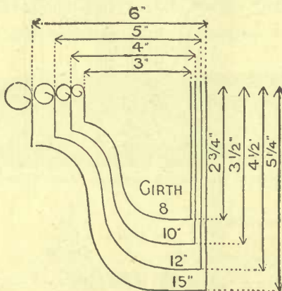
Sections showing dimensions of each size.
